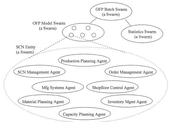
Fig. 5. The implementation of SCNs in Swarm.
