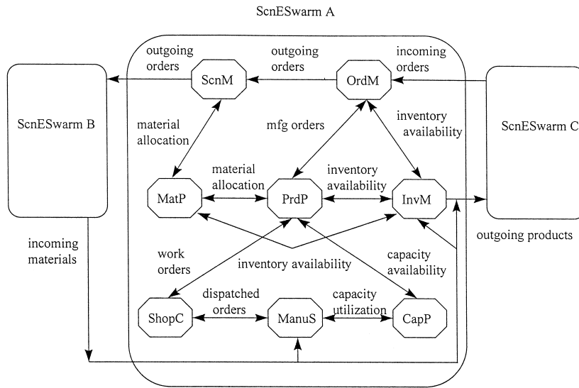
Fig. 6. SCN agent interactions in the Swarm implementation.
